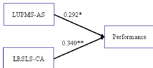
Figure 2. Regression model with explanatory variables obtained through a stepwise regression Testing of Hypotheses
